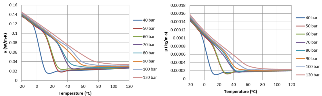
Figure 2.9 Transport properties of CO 2 refrigerant
