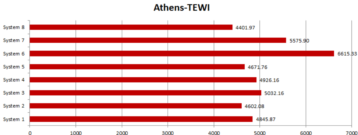
Figure 8.18 TEWI for Athens based on the eight on the investigated cases
