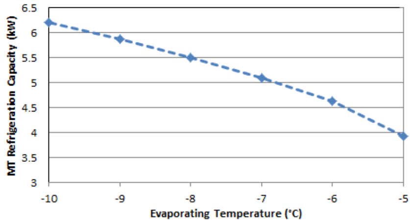
Figure 6.22 Refrigeration capacity for different evaporating temperatures
