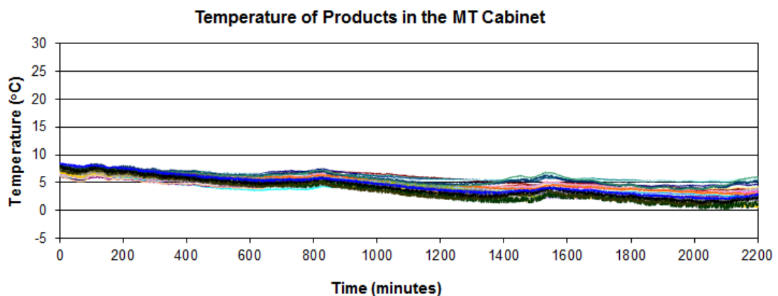
Figure 6.19 Product temperatures
