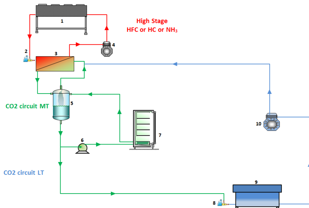
Figure 3.8 Typical subcritical cascade system arrangement
