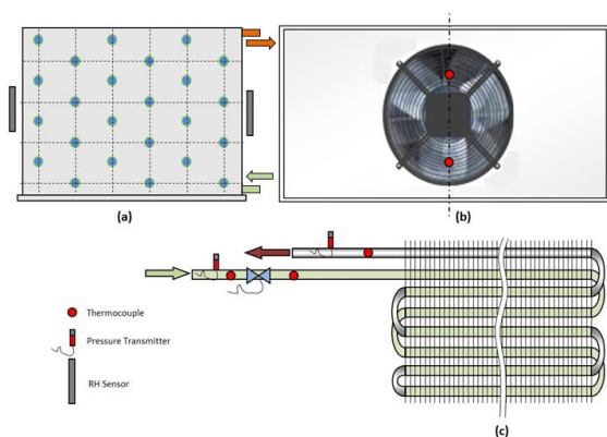
Figure 5.30 AAC unit
