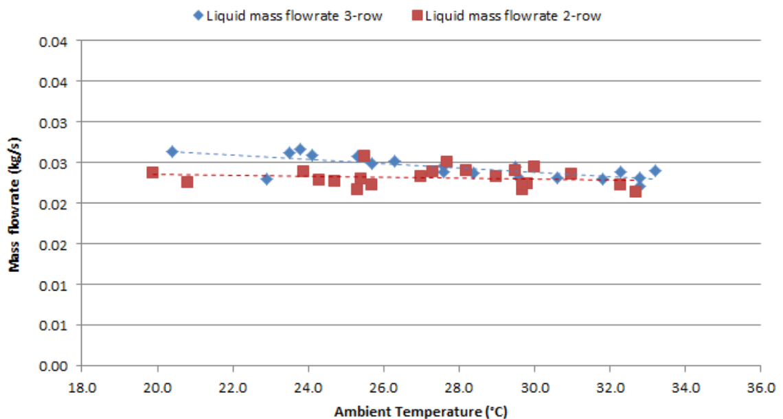
Figure 6.12 Refrigerant liquid flows to both evaporators for different ambient conditions
