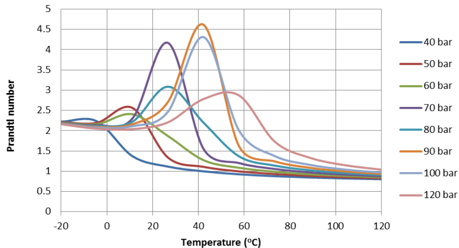
Figure 2.10 CO 2 Prandtl number under different temperatures
